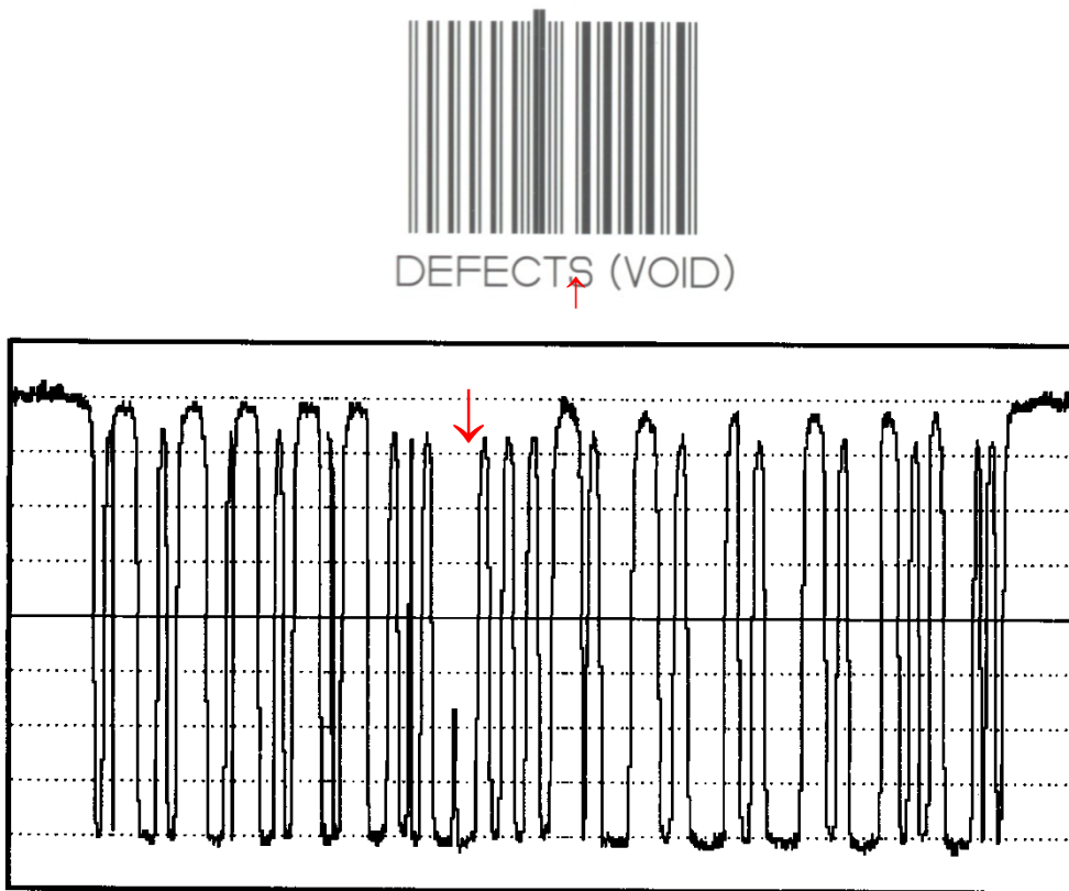
Figure 10-3 : Calibration symbol with engineered defect and associated Scan Reflectance Profile showing defect
