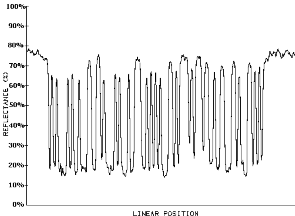
Figure 8-1 : Scan reflectance profile of a UPC-A Barcode
