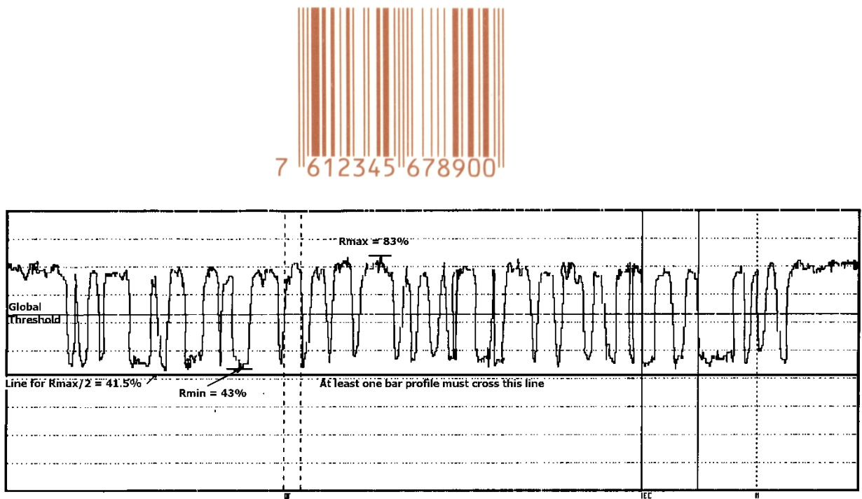
Figure 8-9: Symbol with failing minimum reflectance and associated Scan Reflectance Profile showing failure to meet R_{min} criterion
