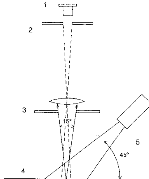
Figure 8-2 : Reference optical arrangement (1 Light sensor, 2 Aperture, 3 Optical obstruction, 4 Verified sample, 5 Light source)
