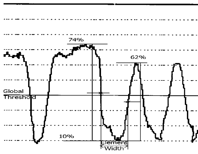
Figure 8-5 : Illustration of edge location in a profile
