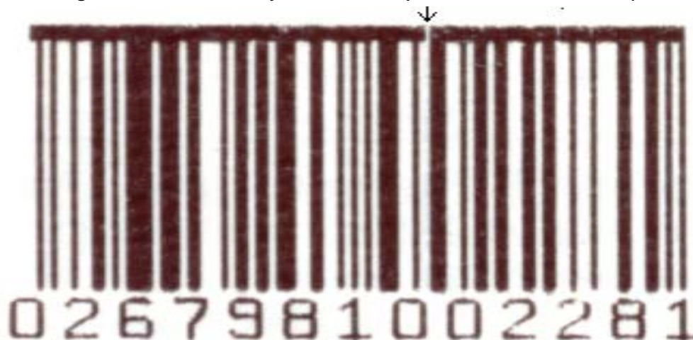
Figure 6-1 : Line above symbol to detect print-head element failure (indicated by arrow)
