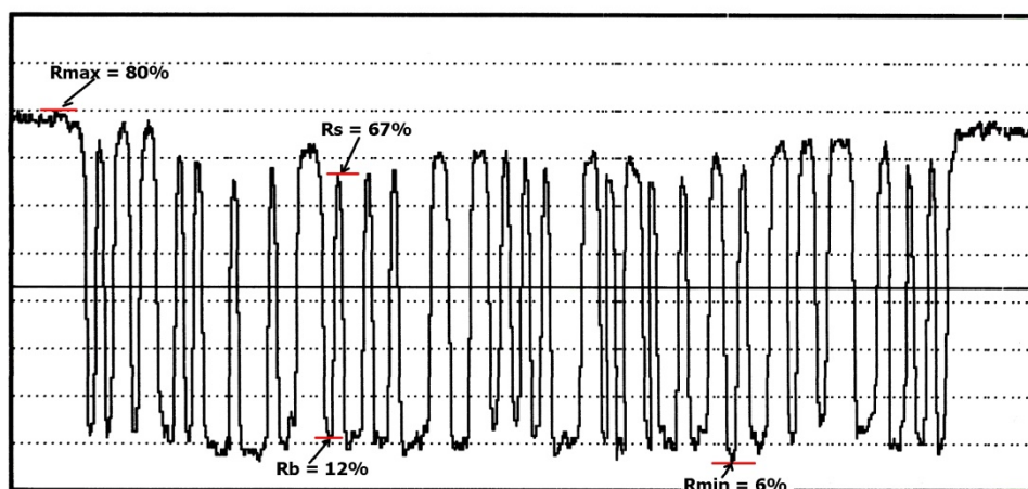
Figure 8-10 : Scan reflectance profile showing edge with lowest Edge Contrast
