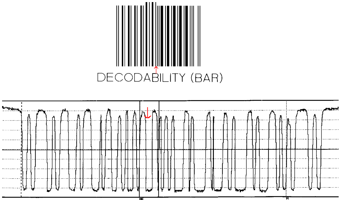
Figure 10-2 : Calibration symbol with engineered low Decodability grade and associated Scan Reflectance Profile of symbol with low Decodability character
