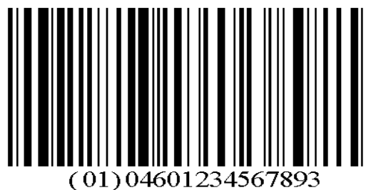
Figure 12-2 : GS1-128 Symbol
