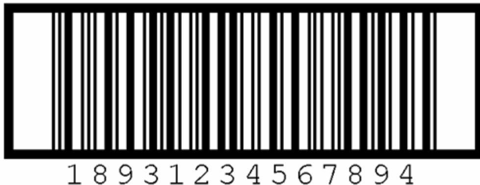
Figure 12-3 : ITF-14 Symbol
