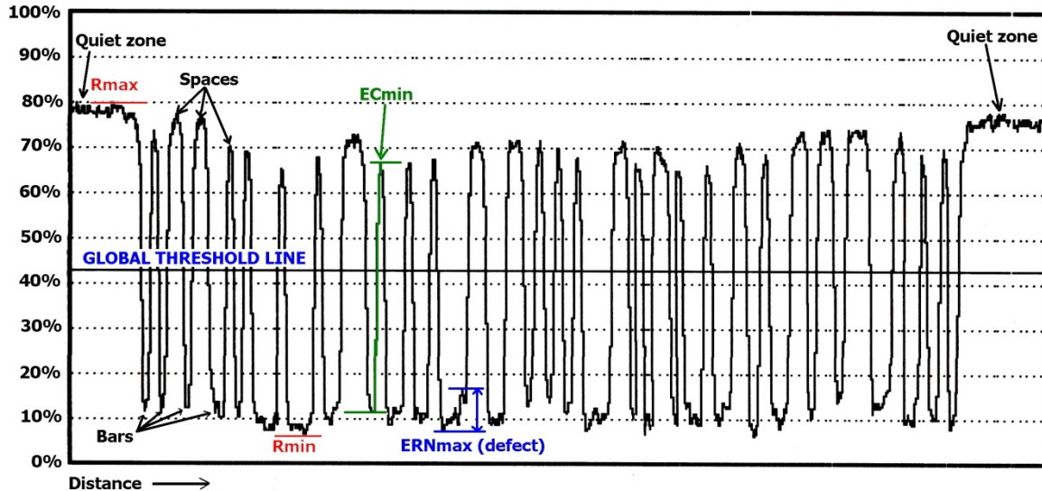
Figure 8-8 : Scan reflectance profile with key measurements indicated
