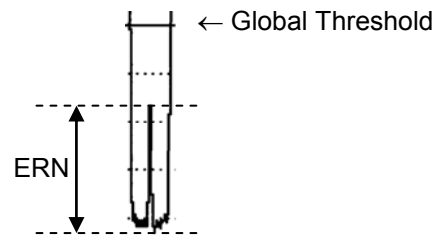
Figure 8-11 : Scan reflectance profile of a bar with a Grade 1 defect
